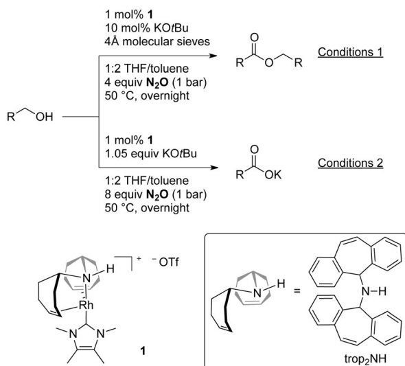
Scheme 1. The two optimized procedures for the formation of esters (conditions 1, top) and carboxylates (conditions 2, bottom) from primary alcohols by dehydrogenative coupling reactions with N 2 O as the hydrogen acceptor.
