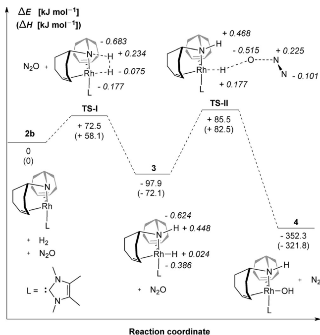
Scheme 4. PBE0/TZVPP electronic-energy differences (in kJ mol -1 ) and enthalpy differences at 323.15 K (in parentheses, in kJ mol -1 ) for H 2 heterolytic addition and the activation and splitting of N 2 O at rhodium complex 2b . NBO charges for the Rh and N atoms and H 2 and N 2 O molecules in TS-I , 3 , and TS-II are given in italics.
